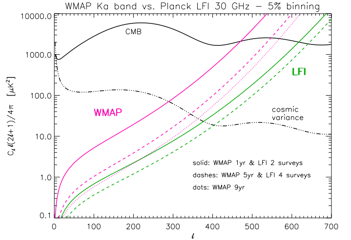
Figure 1. CMB temperature anisotropy APS (black solid line) compatible with WMAP data is compared to WMAP (Ka band) and LFI (30 GHz) sensitivity to the APS (Knox 1995), assuming subtracted the noise expectation, for different integration times as reported in the figure. The plot reports separately the cosmic variance (black three dot-dashes) and the instrumental noise (red and green lines for WMAP and LFI, respectively) assuming a multipole binning of 5%. Regarding sampling variance, an all-sky survey is assumed here for simplicity. The use of the CAMB code is acknowledged ( http://camb.info/ ).
