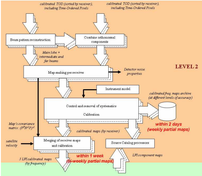
Figure 14. Level 2 MapMaking pipeline.
