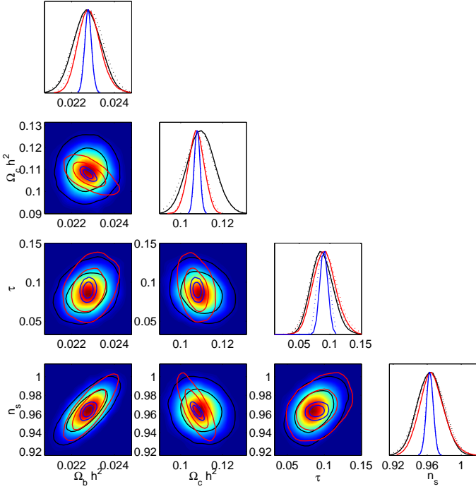
Figure 5. Forecasts of 1\sigma and 2\sigma contours for the cosmological parameters of the WMAP5 best-fit \tau\Lambda CDM cosmological model as expected from Planck (blue lines) and from LFI alone (red lines) after 14 months of observations. The black contours are those obtained from WMAP five years observations. See the text for more details.
