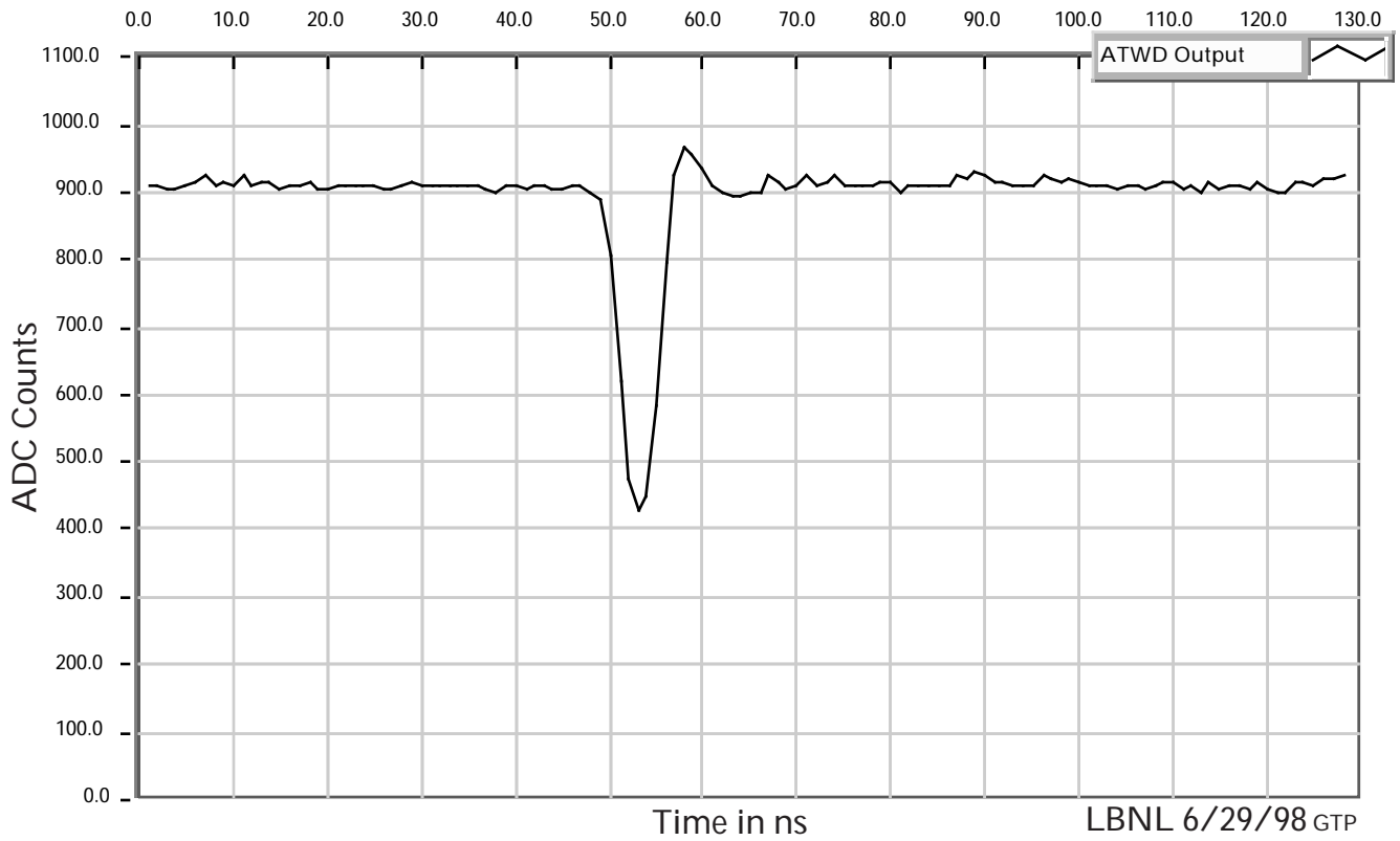
Analogue Transient Waveform Digitizer Response to 1 volt 4 ns wide pulse with sub-nanosecond rise time.
